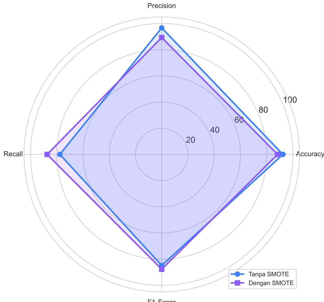
Decision Tree
