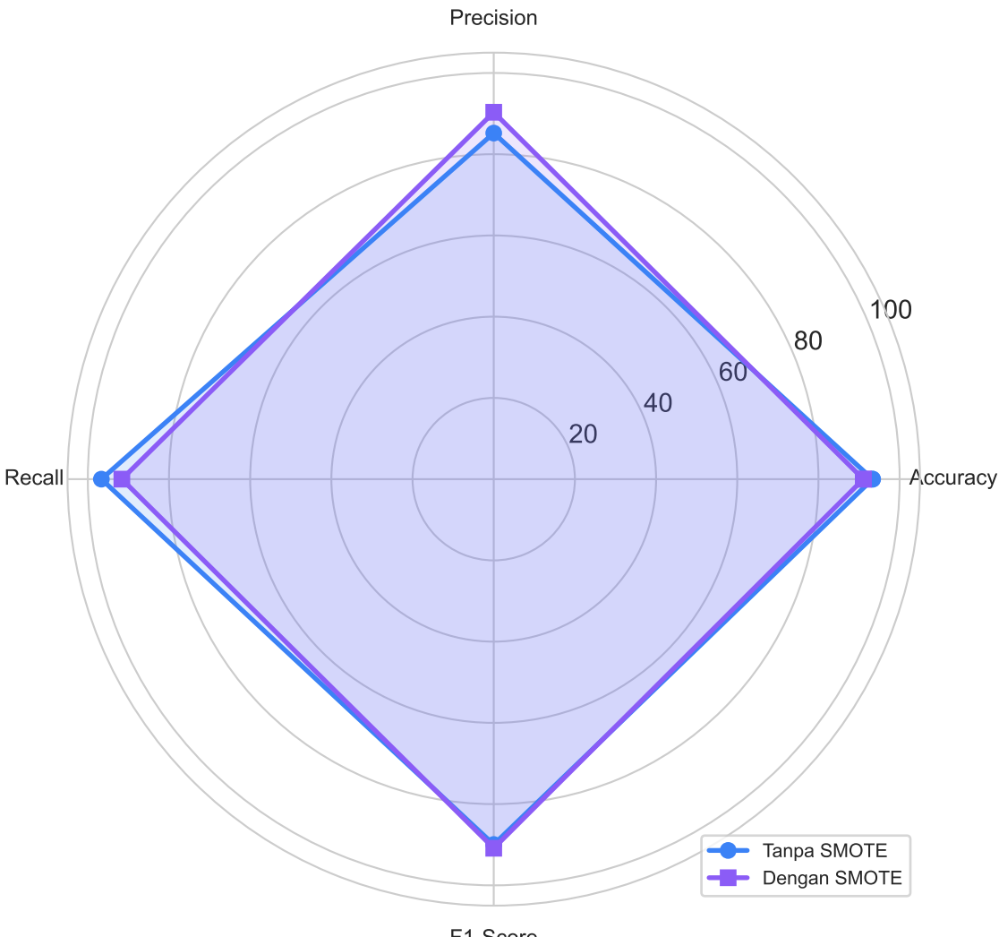
Logistic Regression
