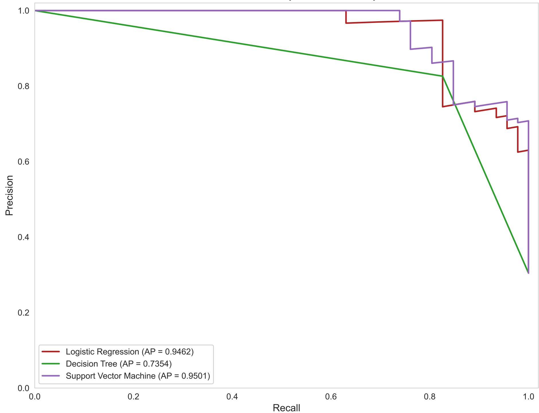
Precision-Recall Curve Comparison for Multiple Models
