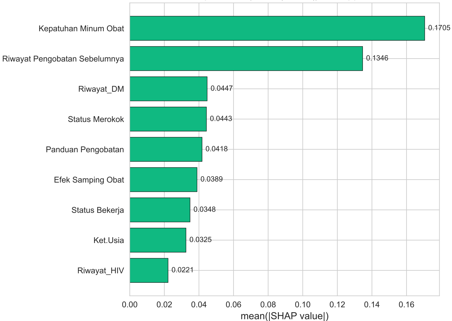
SHAP Feature Importance (mean |SHAP|) — Support Vector Machine
