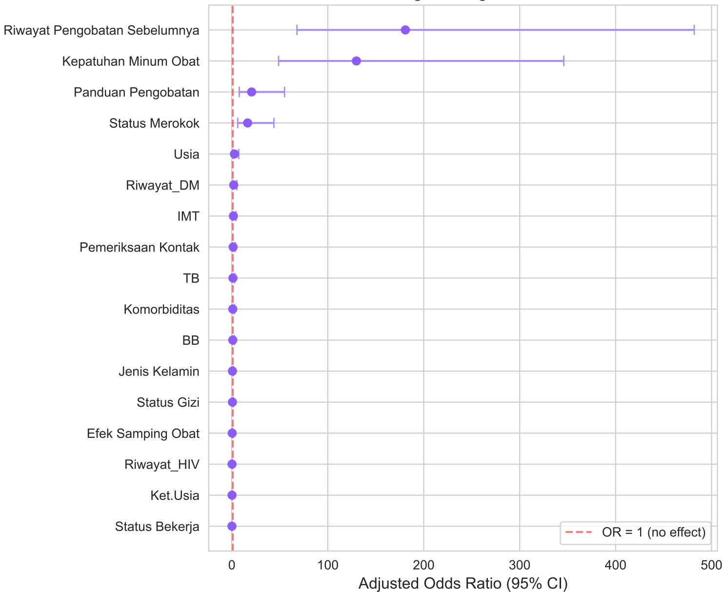
Forest Plot — Logistic Regression Odds Ratios
