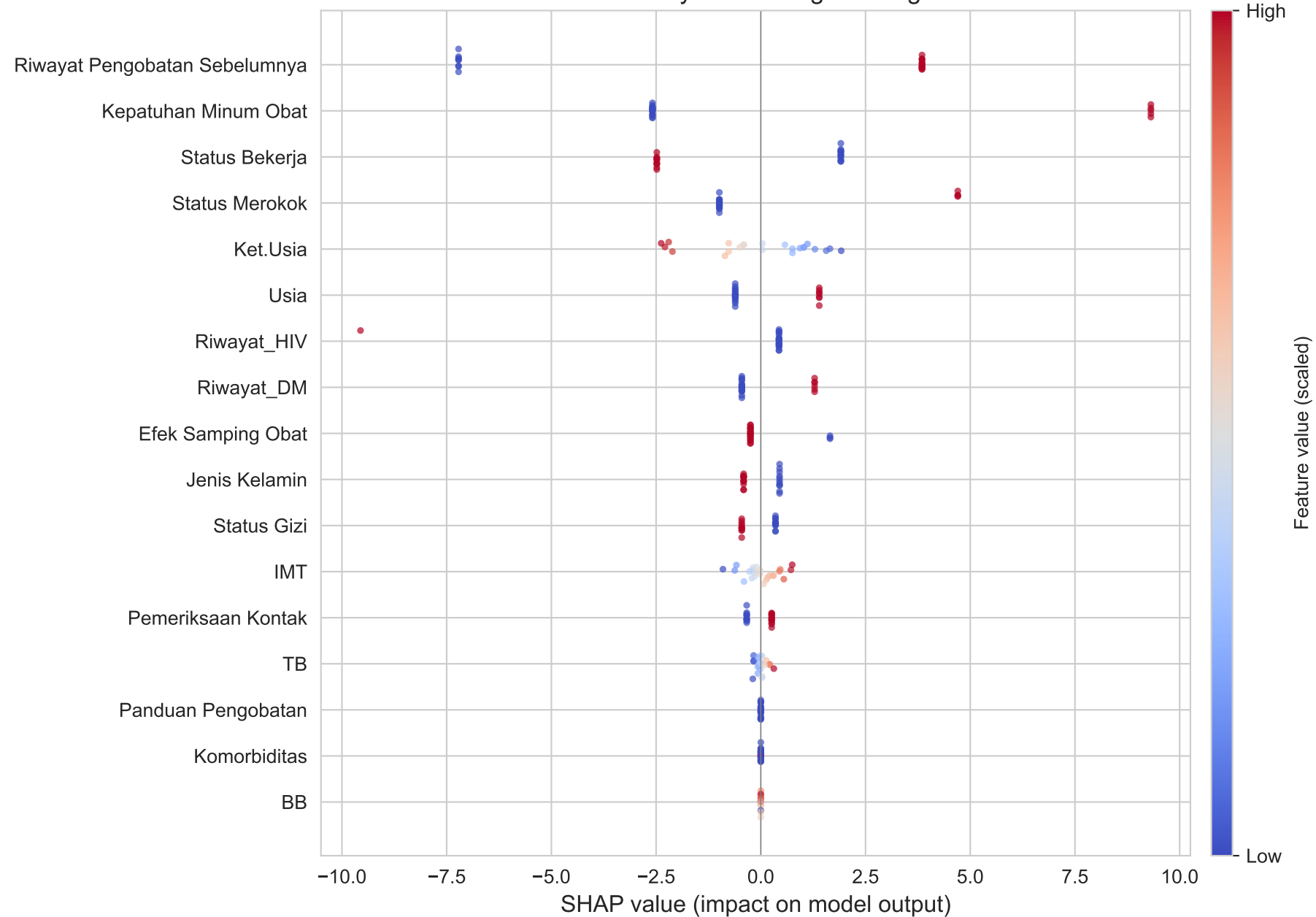
SHAP Summary Plot — Logistic Regression
