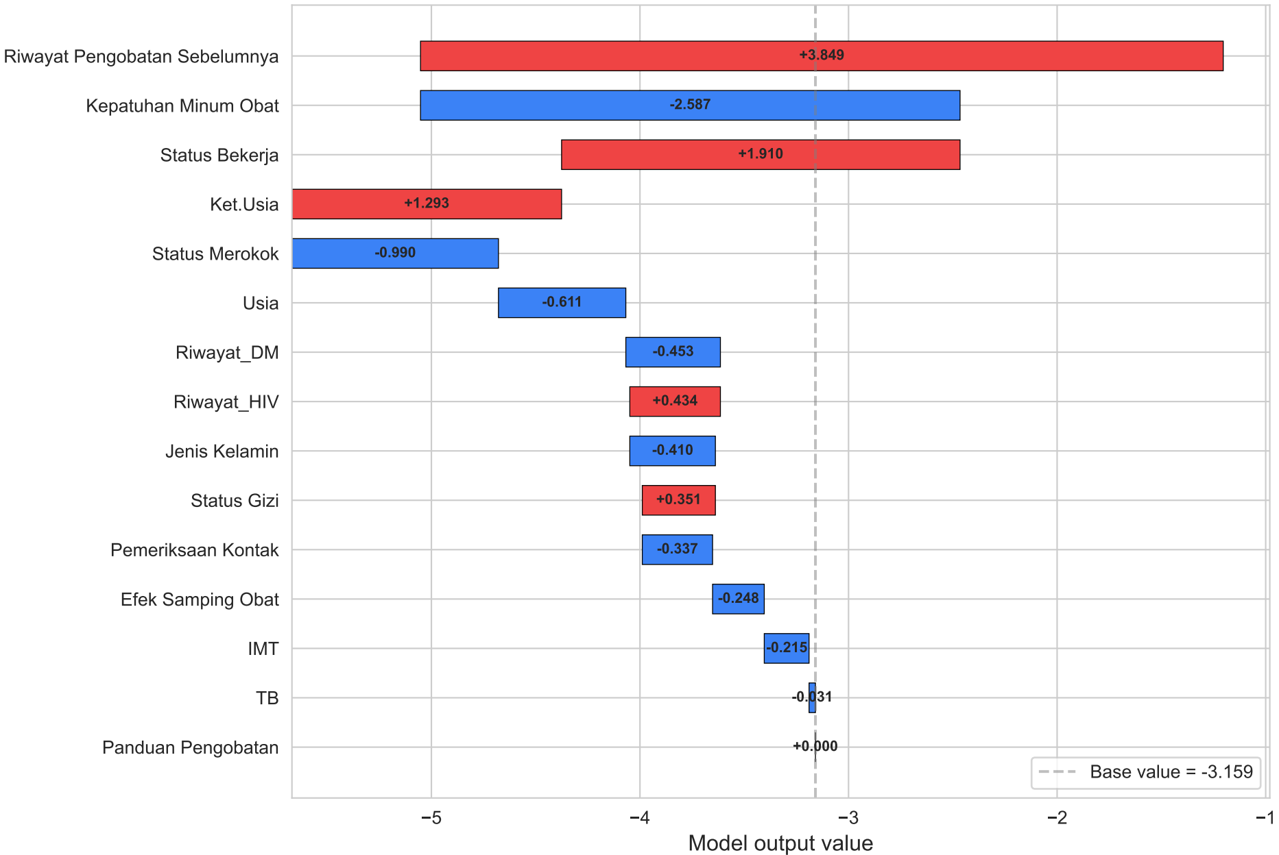
SHAP Waterfall Plot — Logistic Regression (Sample #0)
