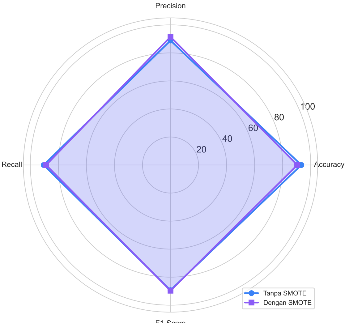
Logistic Regression
