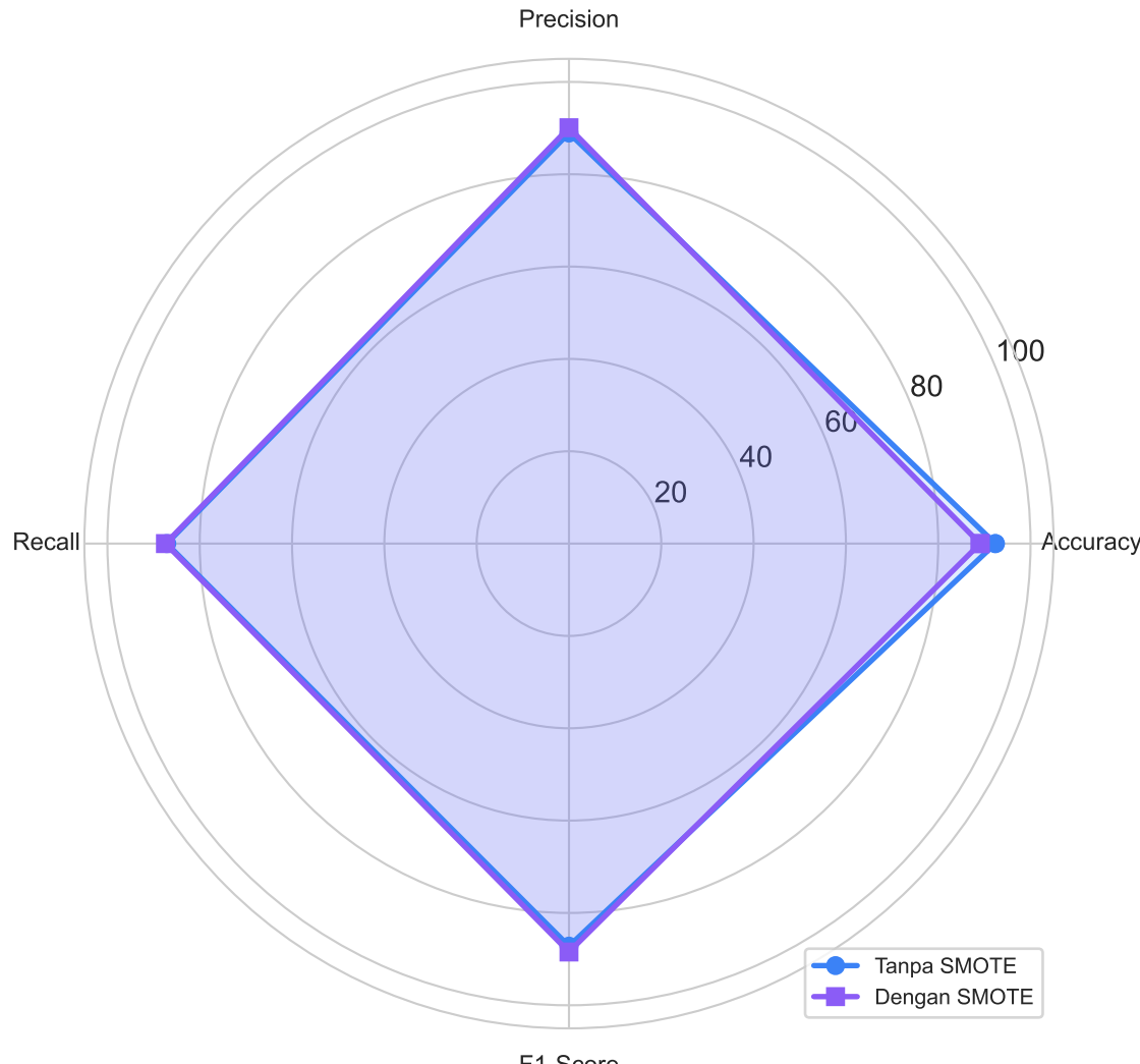
Decision Tree
