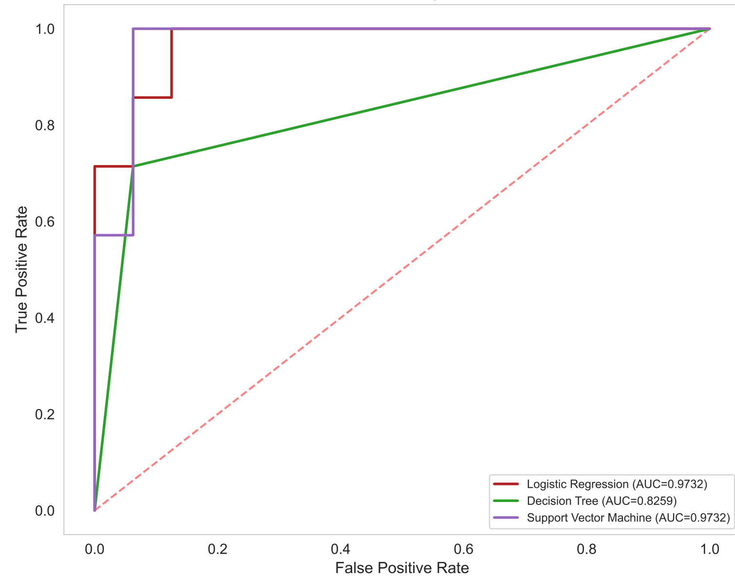
ROC Curve — Tanpa SMOTE
