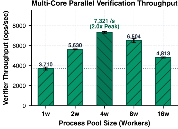
Figure 3: Multi-core parallel policy gate verification throughput across 1, 2, 4, 8, and 16 worker cores. These results confirm that the verification gate scales effectively with multi-core hardware, supporting high-frequency deployment scenarios.
