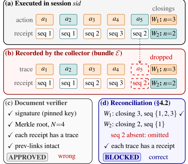
Figure 2: Why a suffix omission is invisible to a document verifier and visible to reconciliation. (a) In session \text{sid} two witnesses, W_1 (orange) and W_2 (teal), serve five actions, returning a sequence-numbered receipt for each and, at session end, a signed closing count. (b) The collector performs all five but records four, dropping a_5 and its receipt; everything it presents is genuine and correctly signed under its own key. (c) A verifier of the document (DSSE, TUF, per-action receipts, hash chains) finds nothing wrong: the end of the record simply moved. (d) The gate reconciles per witness: W_2 ’s closing commits to two served actions but one receipt is present, so the bundle is blocked; producing the missing receipt with a matching trace, or a lower closing, needs W_2 ’s key (Theorem 1).
