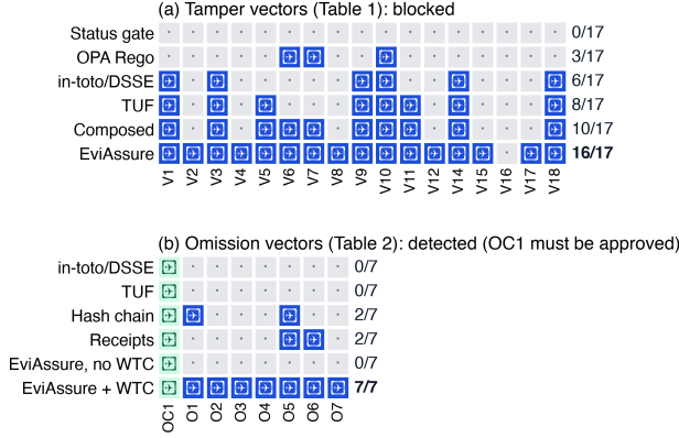
Figure 5: Which vector each verifier stops, read cell by cell from results/security_evaluation.json . (a) The 17 scored tamper vectors of Table 1: what survives the composed pipeline is exactly the trace-level and stateful set (V2, V8, V12, V15, V17, V4); V16 escapes every row. (b) The 7 omission vectors of Table 2: receipts catch only the two attacks that leave an unmatched trace (O5, O6), chaining only the two that break a link (O1, O5); OC1 is approved by every row, as it must be.
