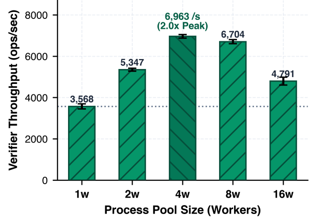
Figure 4: Verifier throughput against process-pool size, mean \pm standard deviation over 5 runs of 1,000 evaluations. The peak bar and its ratio are selected from the data, not fixed to a worker count. Throughput is measured on three-trace bundles and does not describe large- N verification.
