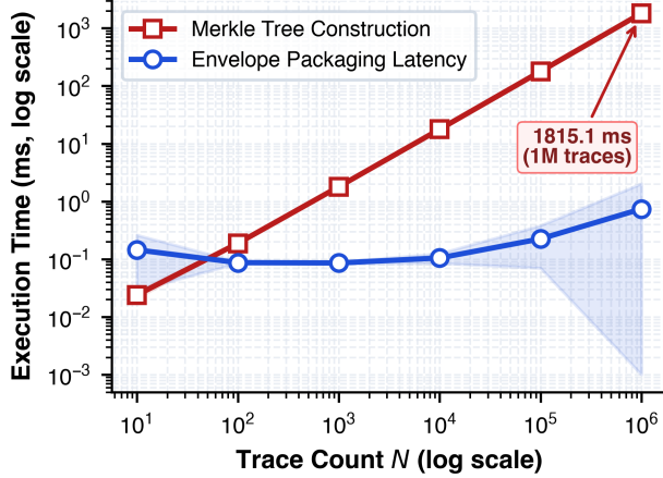
Figure 3: Merkle construction and envelope packaging from N = 10 to N = 10^6 , mean over 5 runs with the standard deviation as a band. Both axes are logarithmic. The callout is read from results/benchmark_summary.json rather than typed, so it cannot diverge from 1815.13 ms in the text.
