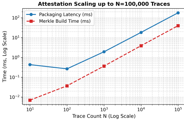
Figure 1: Attestation packaging latency and Merkle tree build time as trace count N scales up to 100,000.
