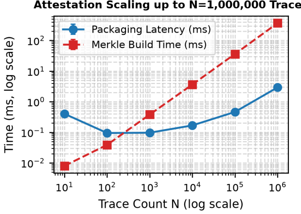
Figure 2 visualizes the performance scaling of the packaging latency and Merkle build time.
