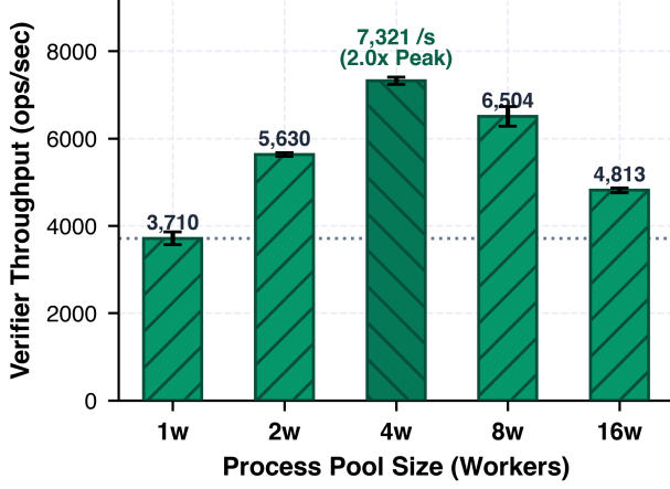
Figure 3 illustrates the verification throughput measured across different multi-core worker pool configurations.
