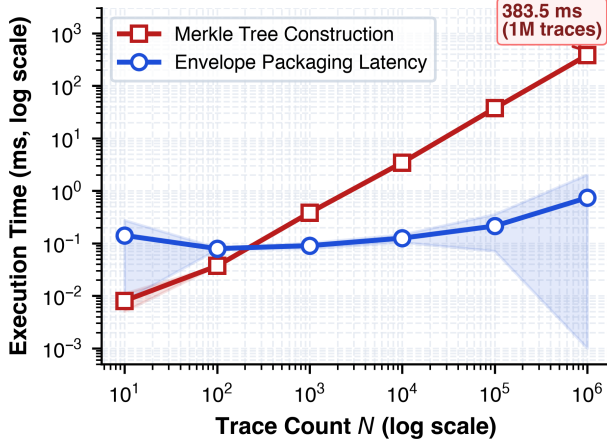
Figure 2 visualizes the performance scaling of the packaging latency and Merkle build time.
