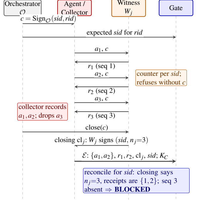
Figure 2: One credentialed session under the witness protocol, and the omission it defeats. The orchestrator opens the session with c and tells the gate which session it credentialed; each action reaches the witness with c and returns a sequence-numbered receipt; at session end the witness signs a closing count. A collector that performs a_3 but records only a_1, a_2 presents a bundle \mathcal{E} (signed under its own key K_C ) whose closing and receipts disagree, and the gate blocks; the missing receipt or a lower closing needs W_j ’s key (Theorem 1).
