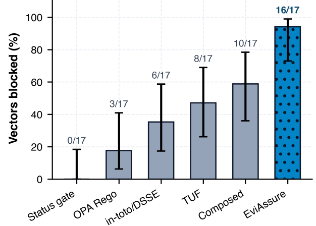
Figure 4: Executed baselines against the 17-vector suite, with Wilson 95% intervals. The intervals overlap, and that is the point: at this sample size the evaluation supports a qualitative account of which vectors survive a modern composed pipeline, not a strong quantitative separation (Section 7.6).
