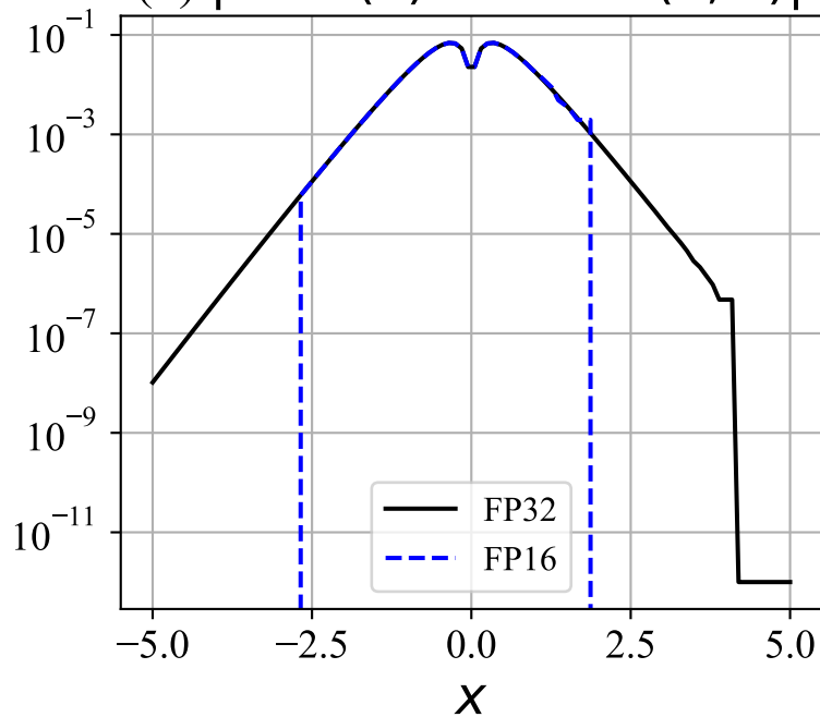
(b) |\text{ReLU}(x) - \text{WSiLU}(x; 4)|
