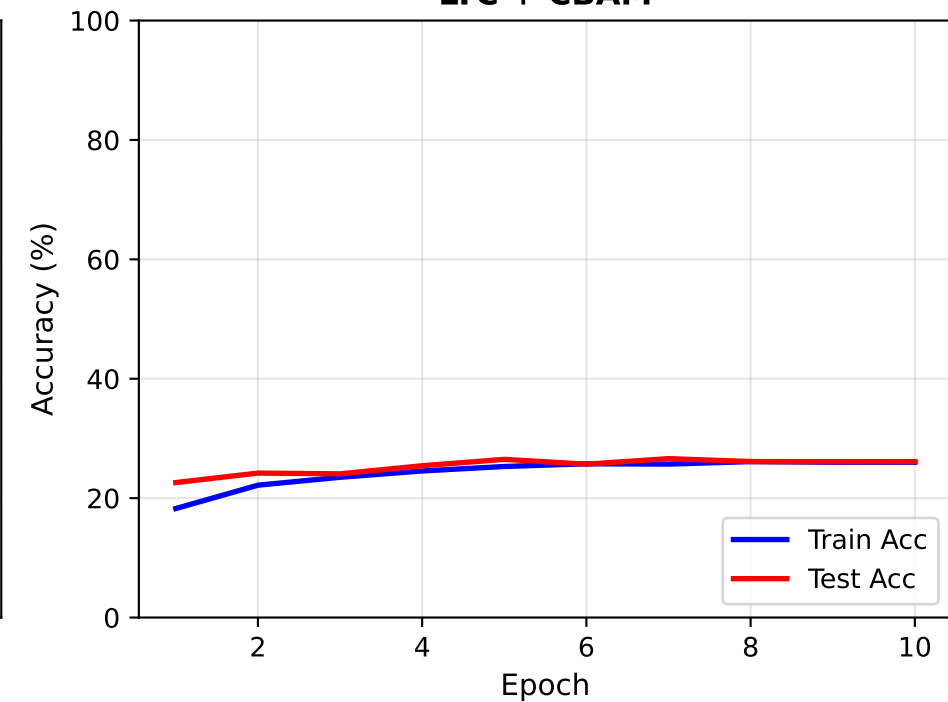
LTC + CBAM
