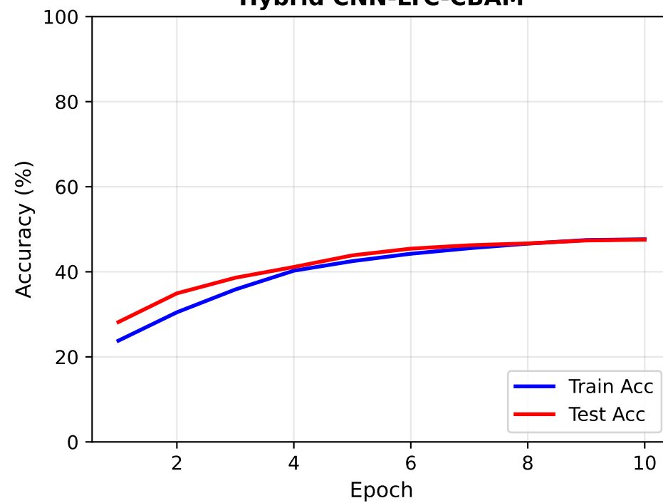
Hybrid CNN-LTC-CBAM
