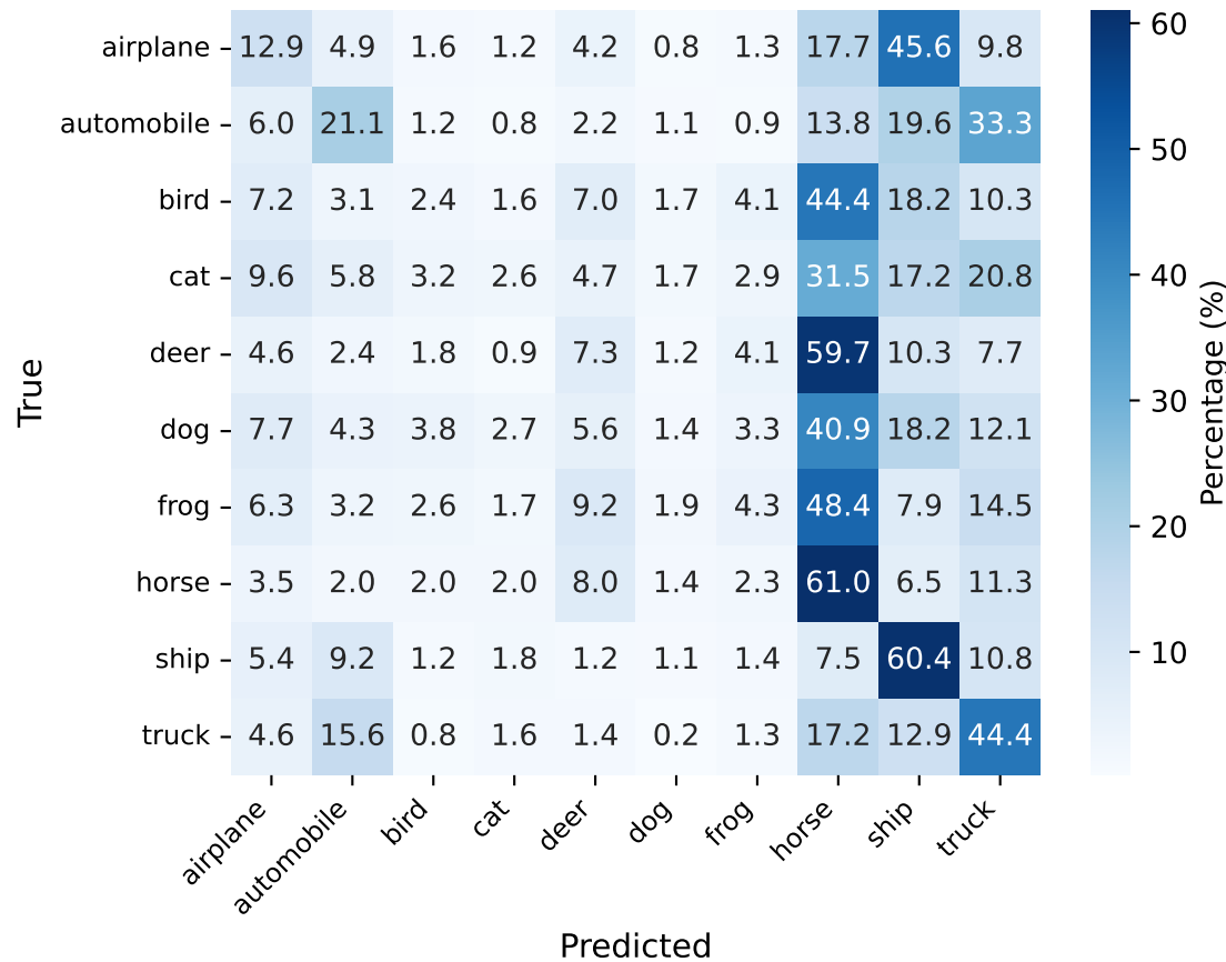
Pure LTC
