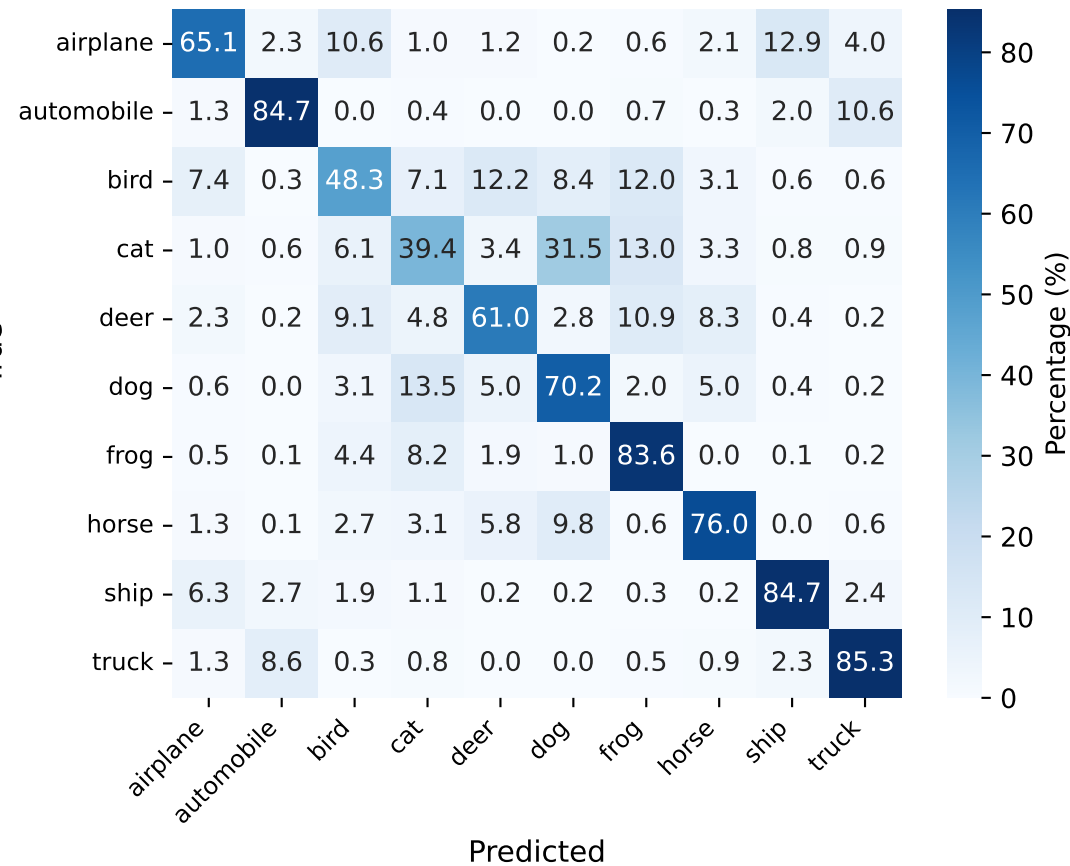
Baseline CNN
