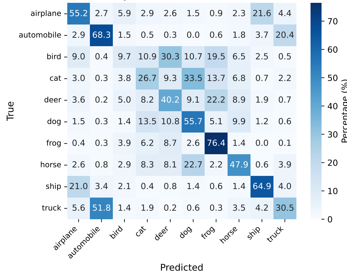
Hybrid CNN-LTC-CBAM
