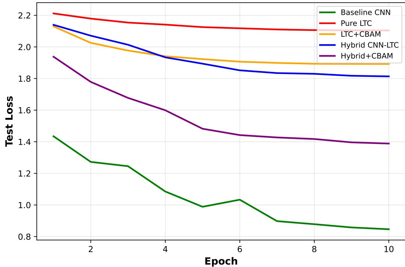
Test Loss Comparison
