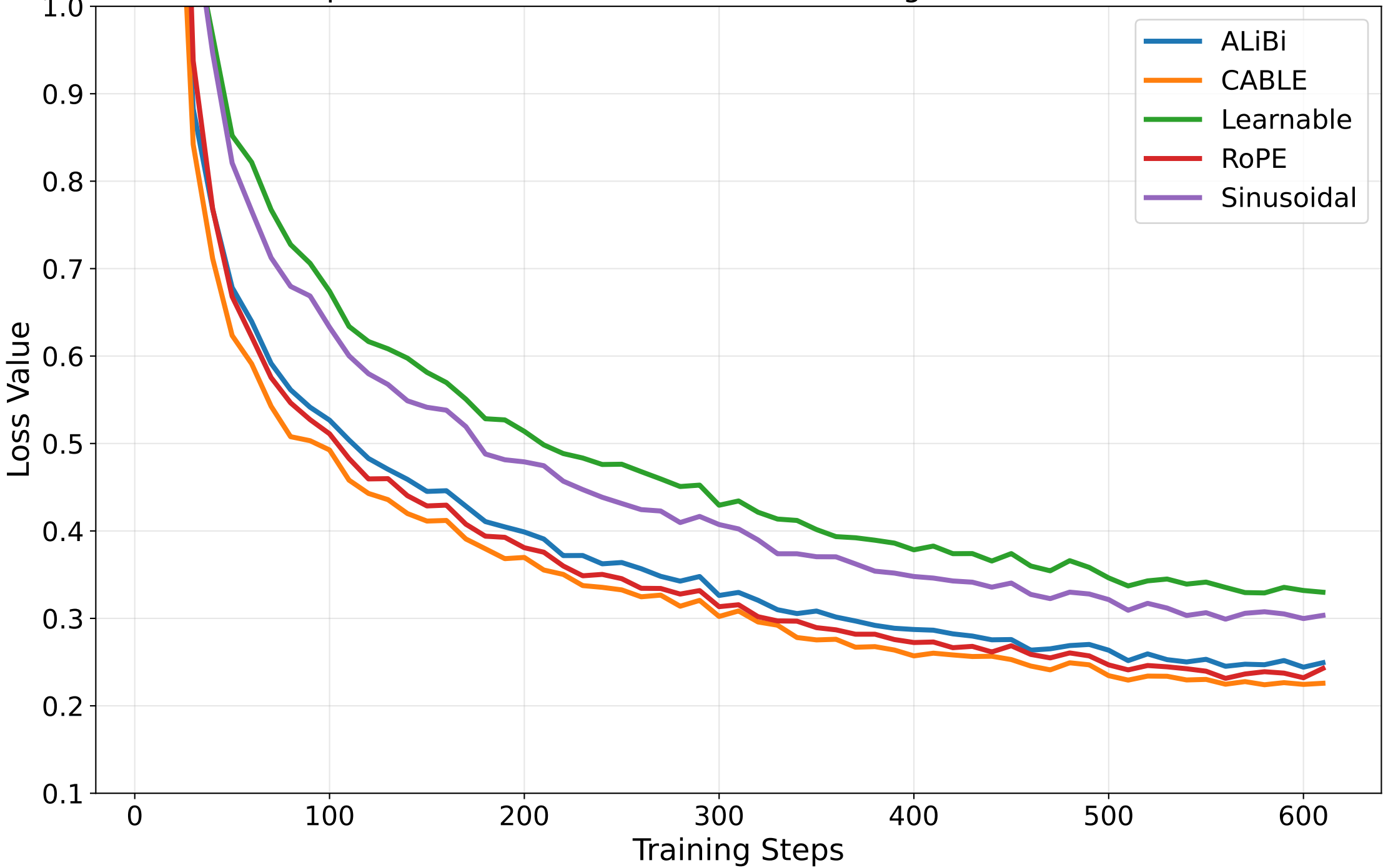
Comparison of BERT Contrastive Fine-tuning Loss on MS-MARCO
