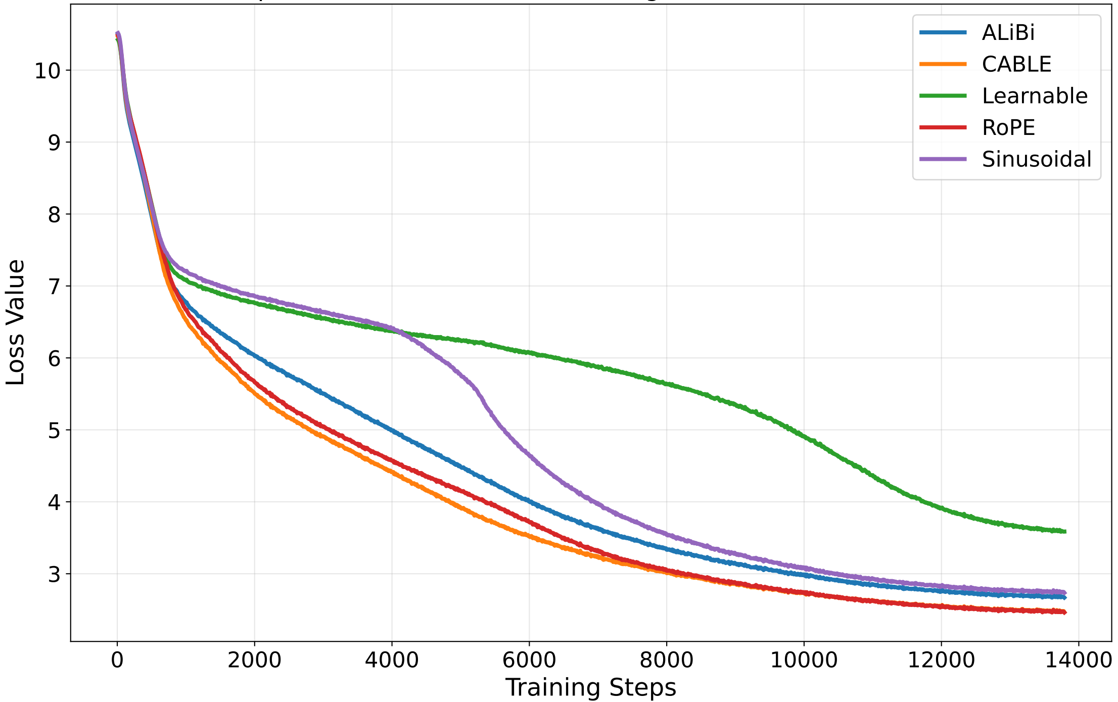
Comparison of BERT MLM Pre-training Loss on FineWeb-Edu-10B
