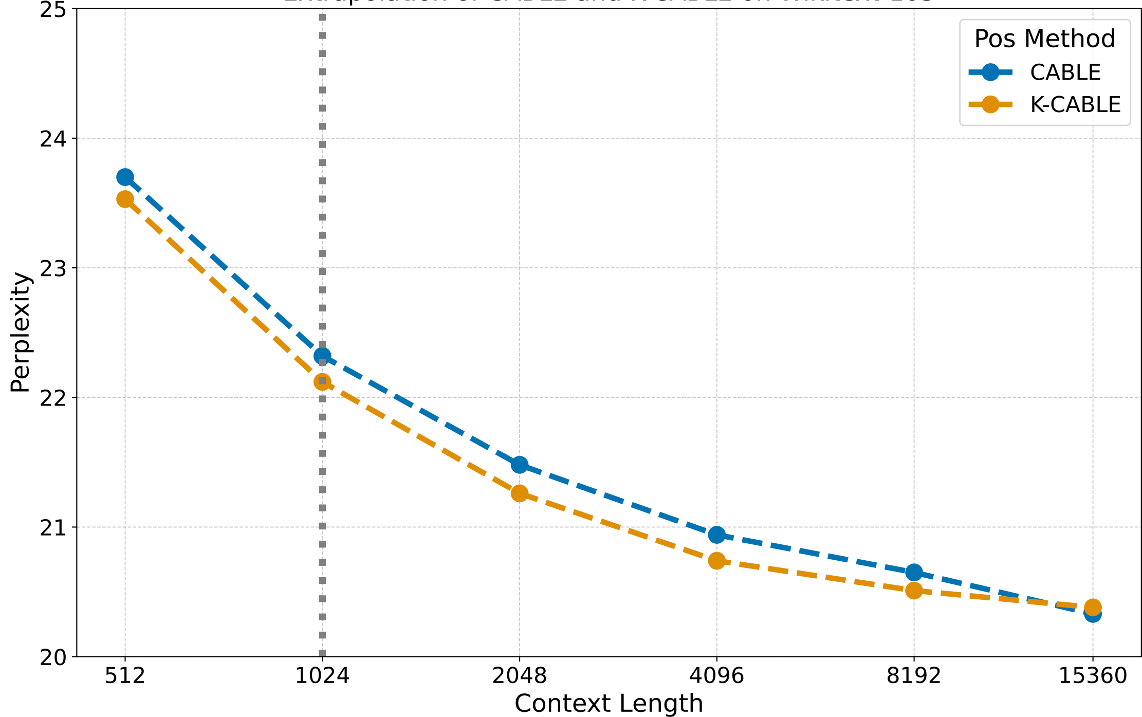
Extrapolation of CABLE and K-CABLE on Wikitext-103
