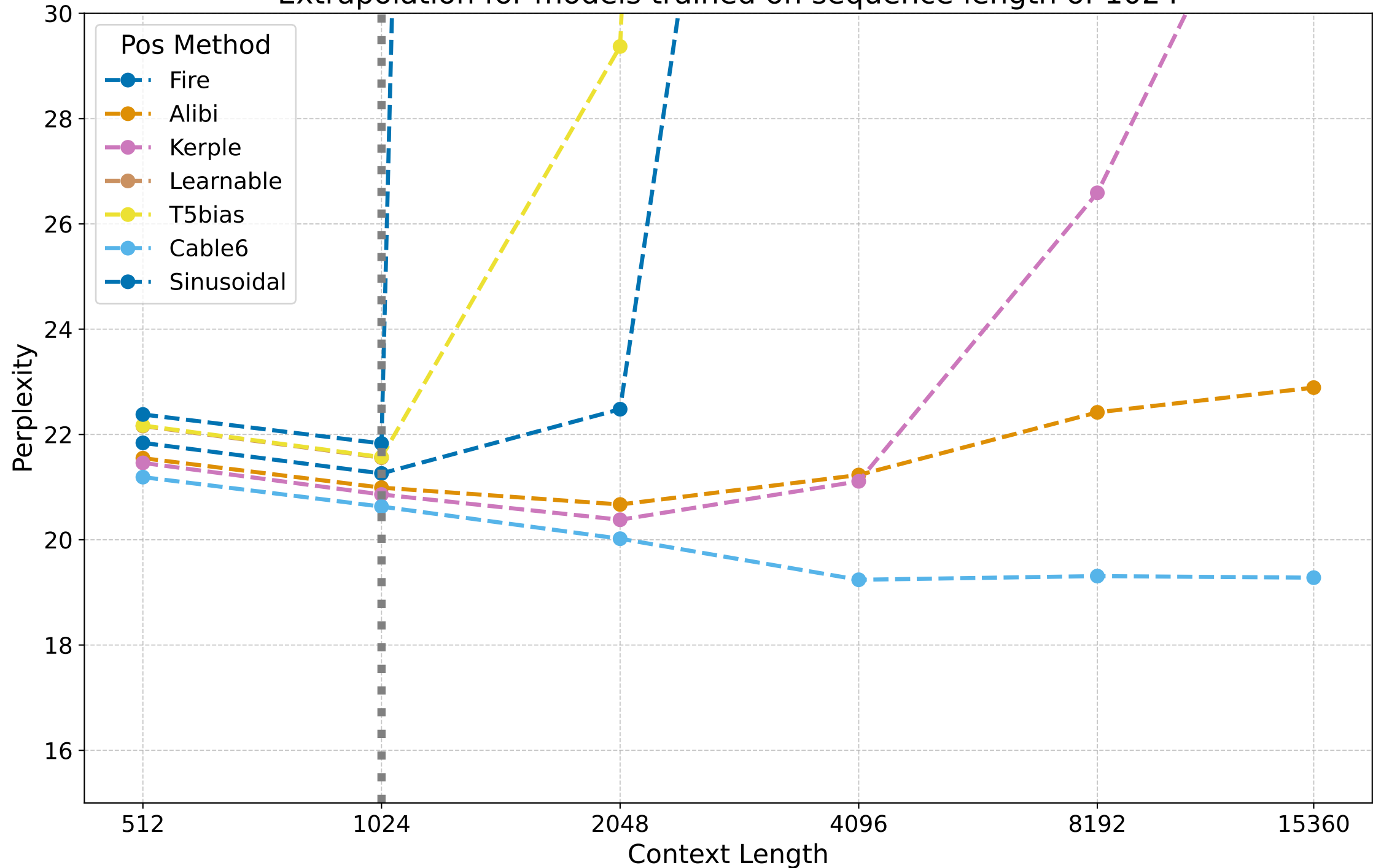
Extrapolation for models trained on sequence length of 1024
