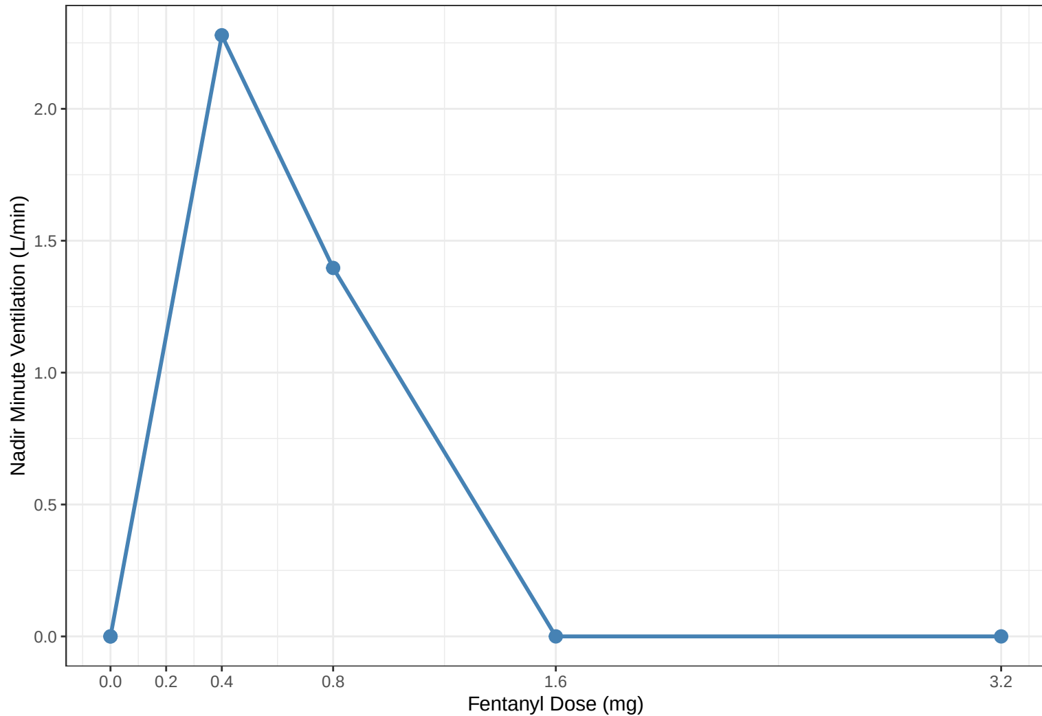
Nadir Minute Ventilation vs Fentanyl Dose (No Naloxone Administration)
