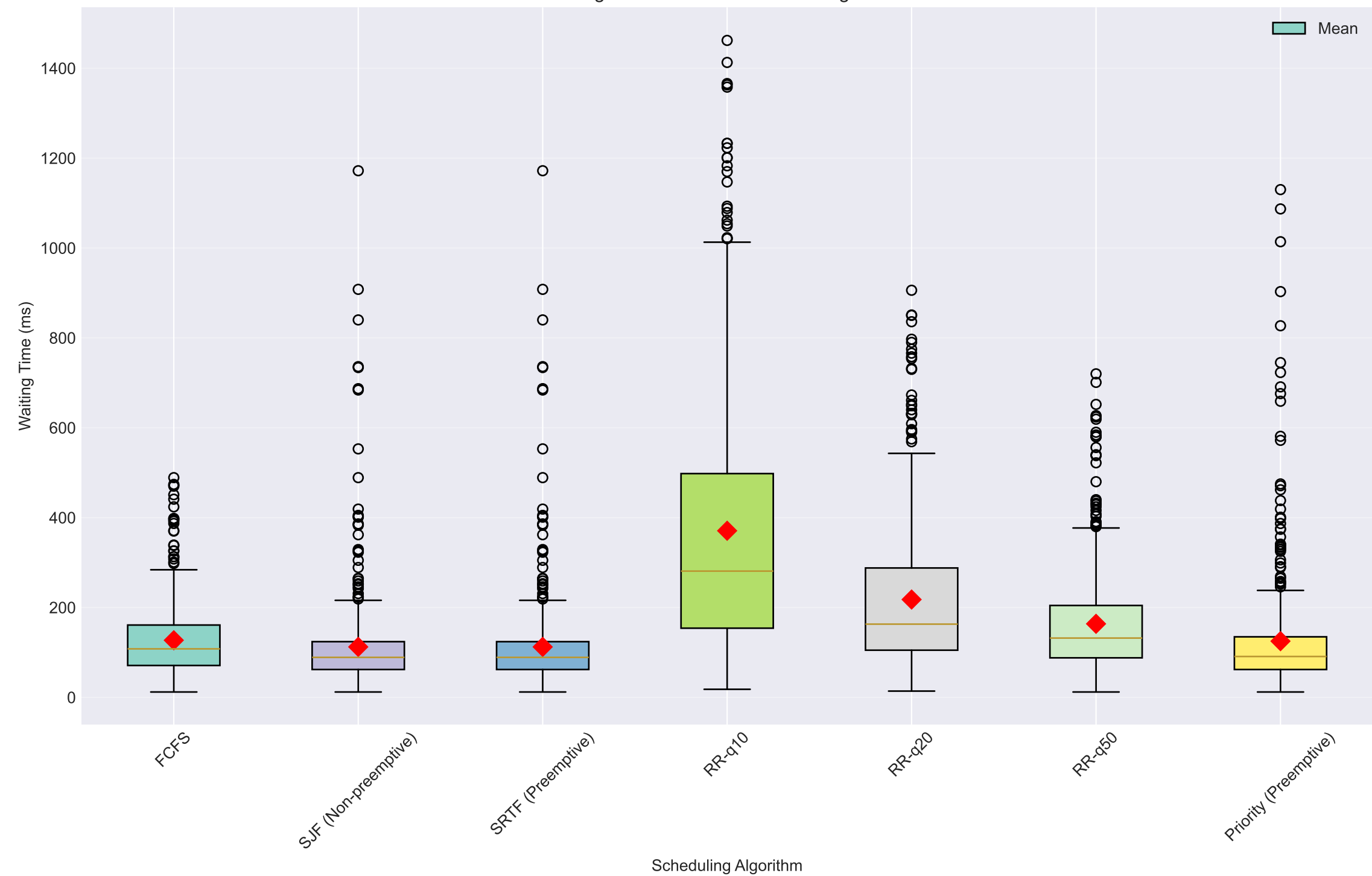
Waiting Time Distribution Across Algorithms
