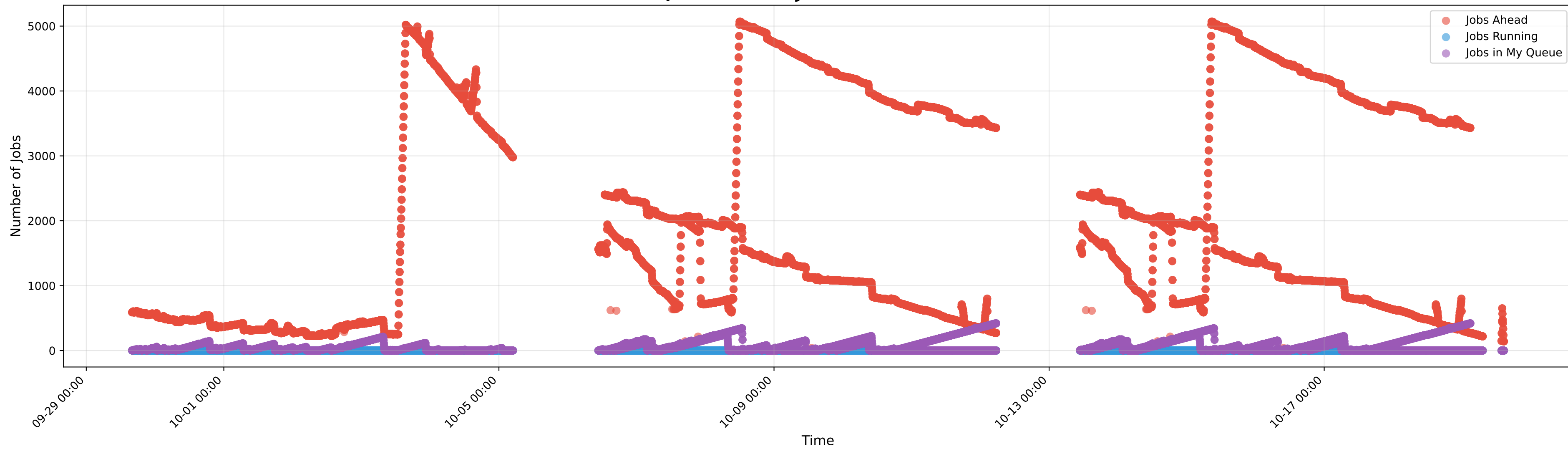
Queuing Delay Over Time by Core Count
