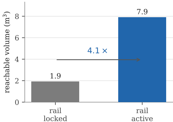
(a) workspace gain from the rail DOF
