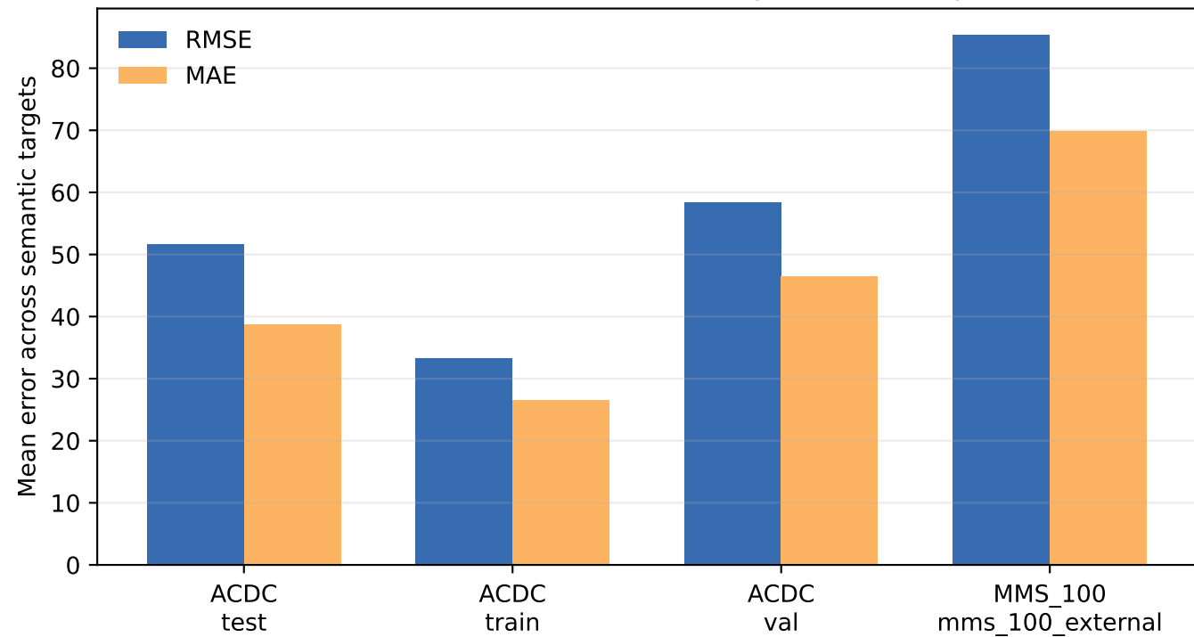
Transition reconstruction error by evaluation split
