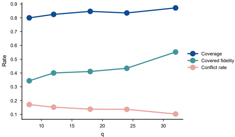
Quantile granularity sensitivity
