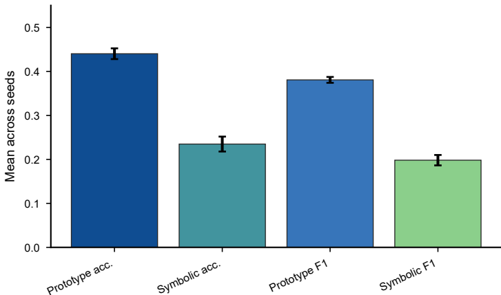
Protocol B semantic-transfer metrics
