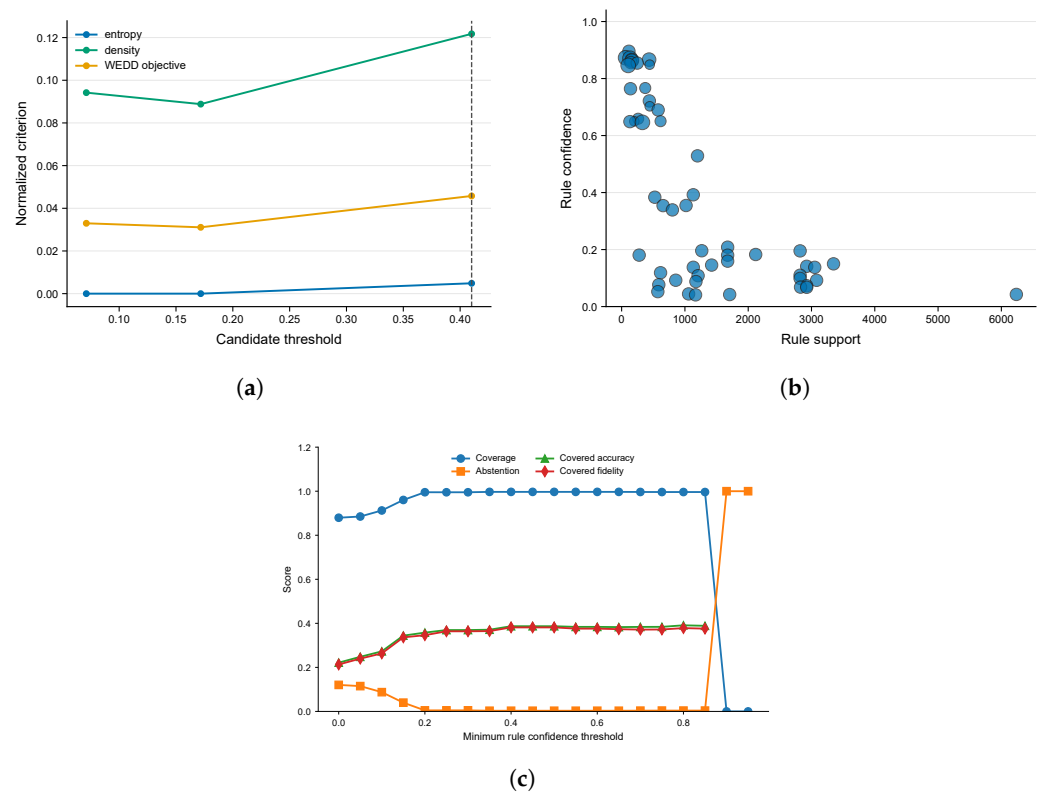
Figure 4. Rulebook and threshold optimization. (a) WEDD threshold example on a selected AwA2 semantic attribute. The plot shows how entropy and density jointly determine an interpretable threshold. (b) Rule support and confidence distribution for the AwA2 Protocol A rulebook. (c) Coverage, abstention, covered accuracy, and covered fidelity as the minimum rule-confidence threshold varies.
