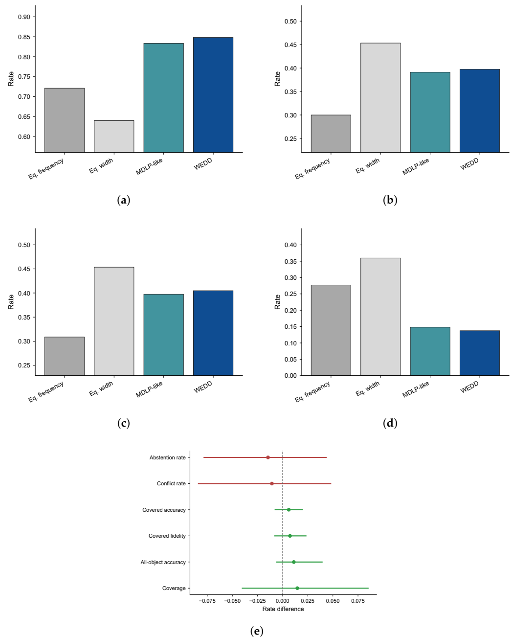
Figure S4. Discretizer evidence across coverage, accuracy, fidelity, conflict, and paired WEDD-minus-MDLP-like entropy intervals. (a) Coverage by discretizer. (b) Accuracy by discretizer. (c) Fidelity by discretizer. (d) Conflict by discretizer. (e) Paired WEDD-MDLP-like entropy intervals. The panels support cautious framing: the observed WEDD advantages are modest and should be treated as operating-point evidence rather than universal dominance.
