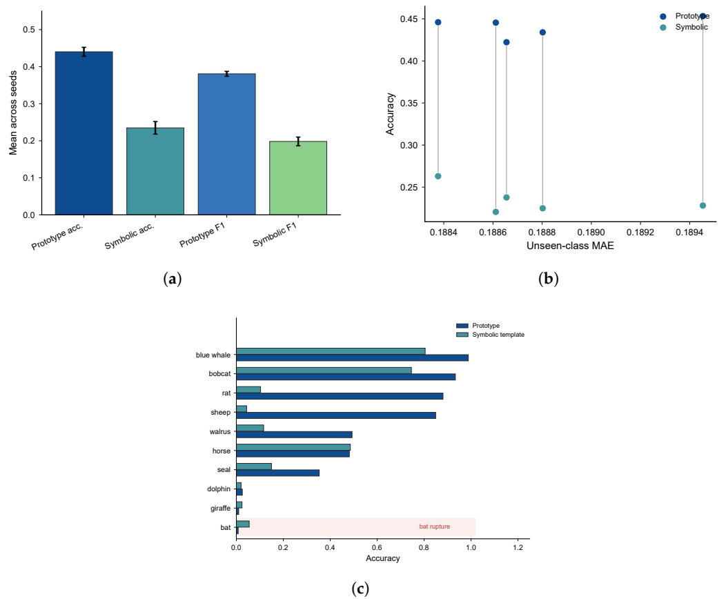
Figure S6. Protocol B semantic-transfer diagnostics. The panels summarize seed-level variation, accuracy-versus-MAE behavior, and per-class failure modes for bat, giraffe, dolphin, and sheep.
