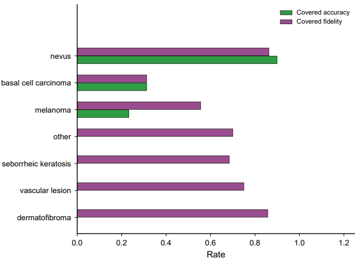
Figure S3. Derm7pt grouped-diagnosis diagnostics under the locked ResNet-50 technical-validation protocol. The figure should not be interpreted as clinical validation.
