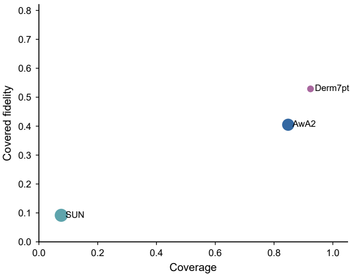
Figure S7. Cross-domain portability viewed through coverage and fidelity. The figure shows that SEMTRA’s audit behavior is strongly dataset-dependent.
