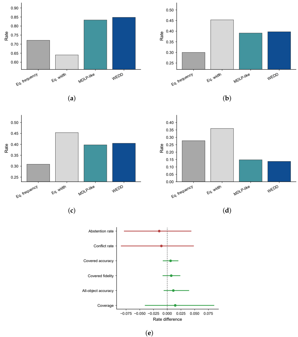
Figure S4. Discretizer evidence across coverage, accuracy, fidelity, conflict, and paired WEDD-minus-MDLP-like entropy intervals. (a) Coverage by discretizer. (b) Accuracy by discretizer. (c) Fidelity by discretizer. (d) Conflict by discretizer. (e) Paired WEDD-MDLP-like entropy intervals. The panels support cautious framing: the observed WEDD advantages are modest and should be treated as operating-point evidence rather than universal dominance.
