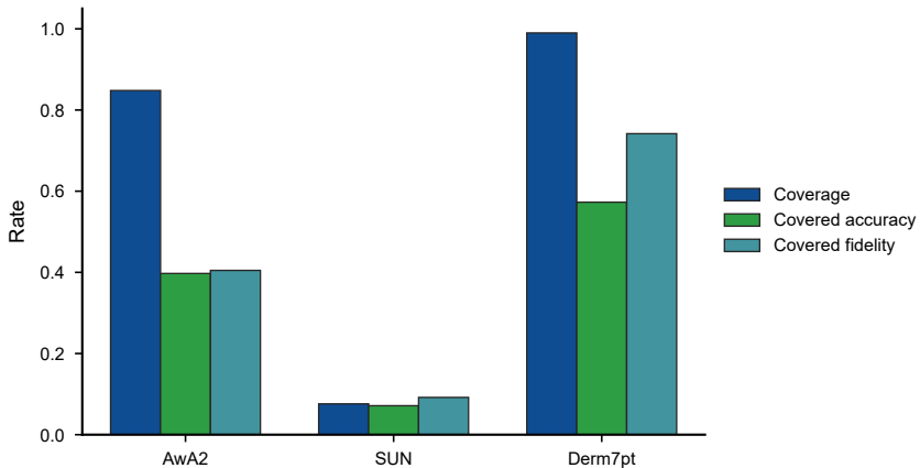
Object-level audit outcomes
