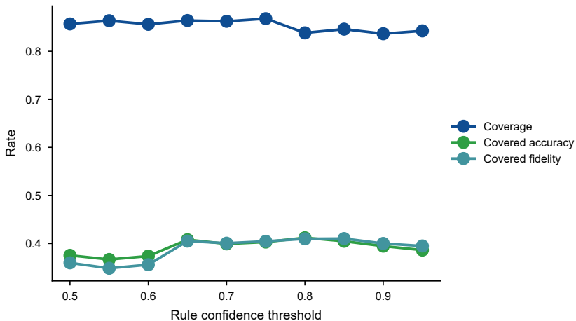
Confidence threshold frontier
