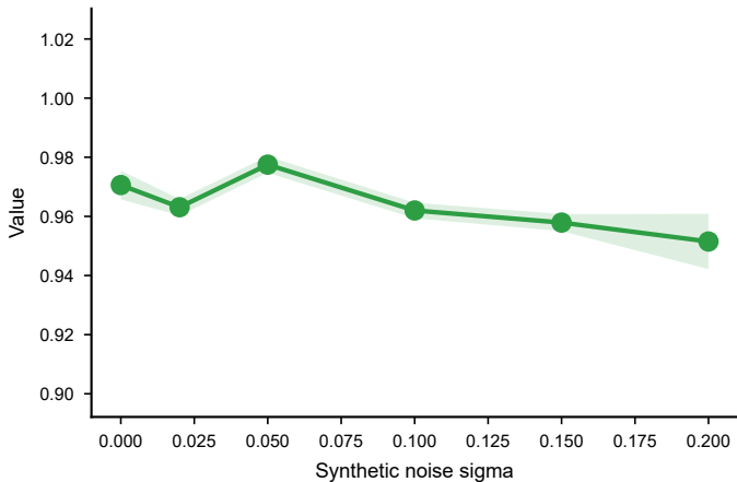
Synthetic coverage under noise
