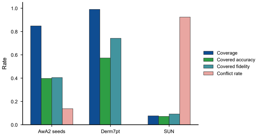
v3 cross-domain object metrics
