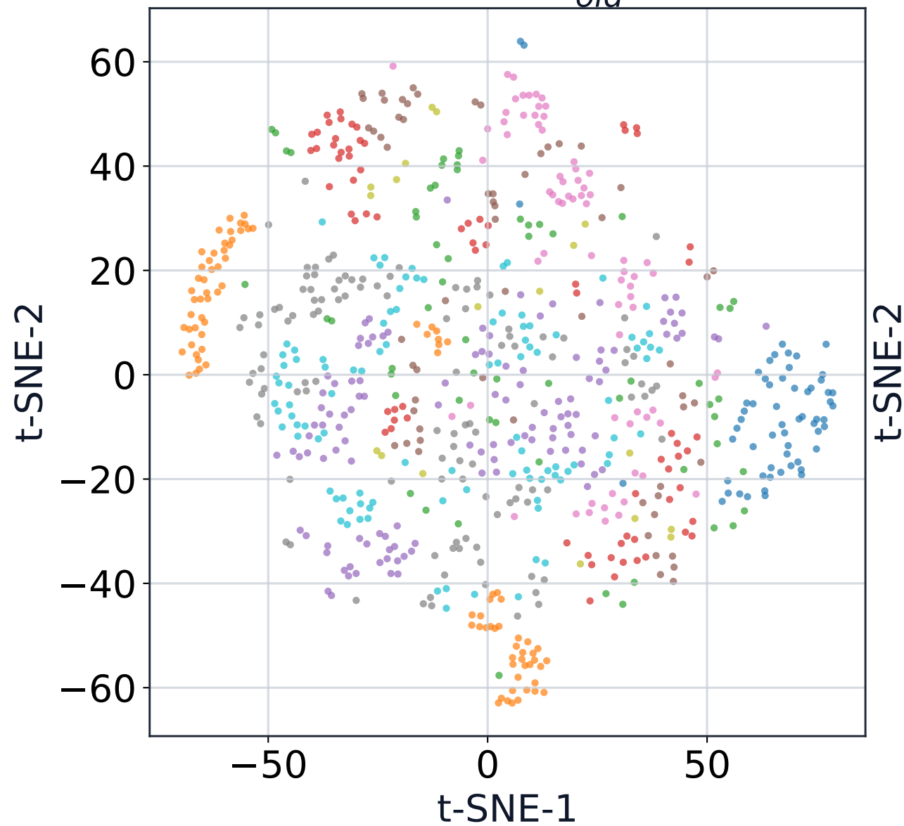
t-SNE: B_{old}^*
