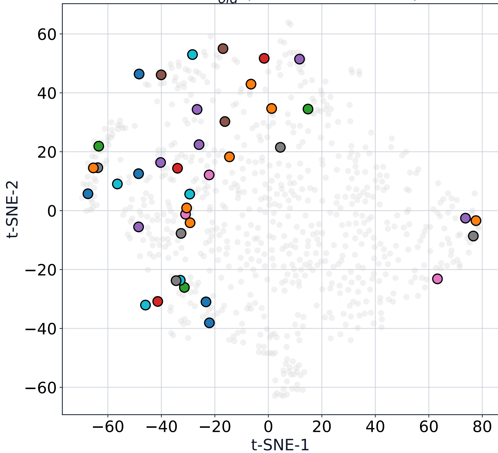
t-SNE: B_{old}^* (Rotated vs Static)
