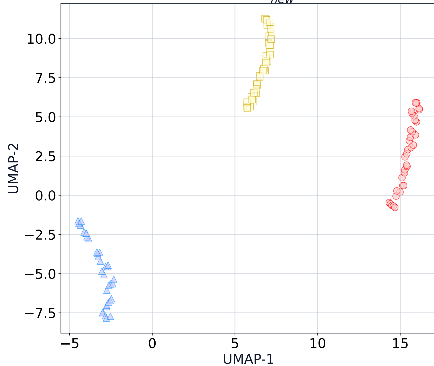
UMAP: B_{new}^*
