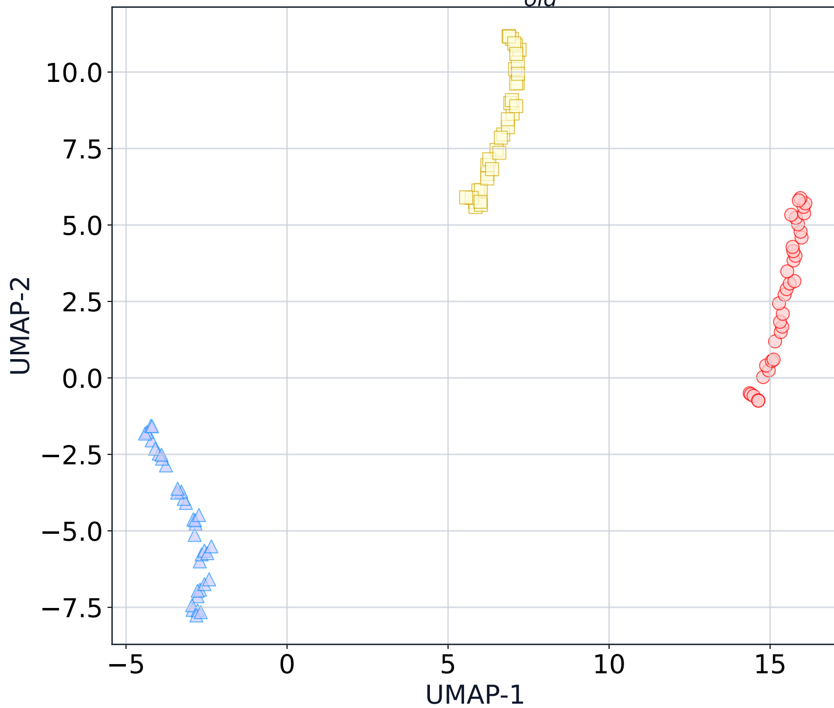
UMAP: B_{old}^*
