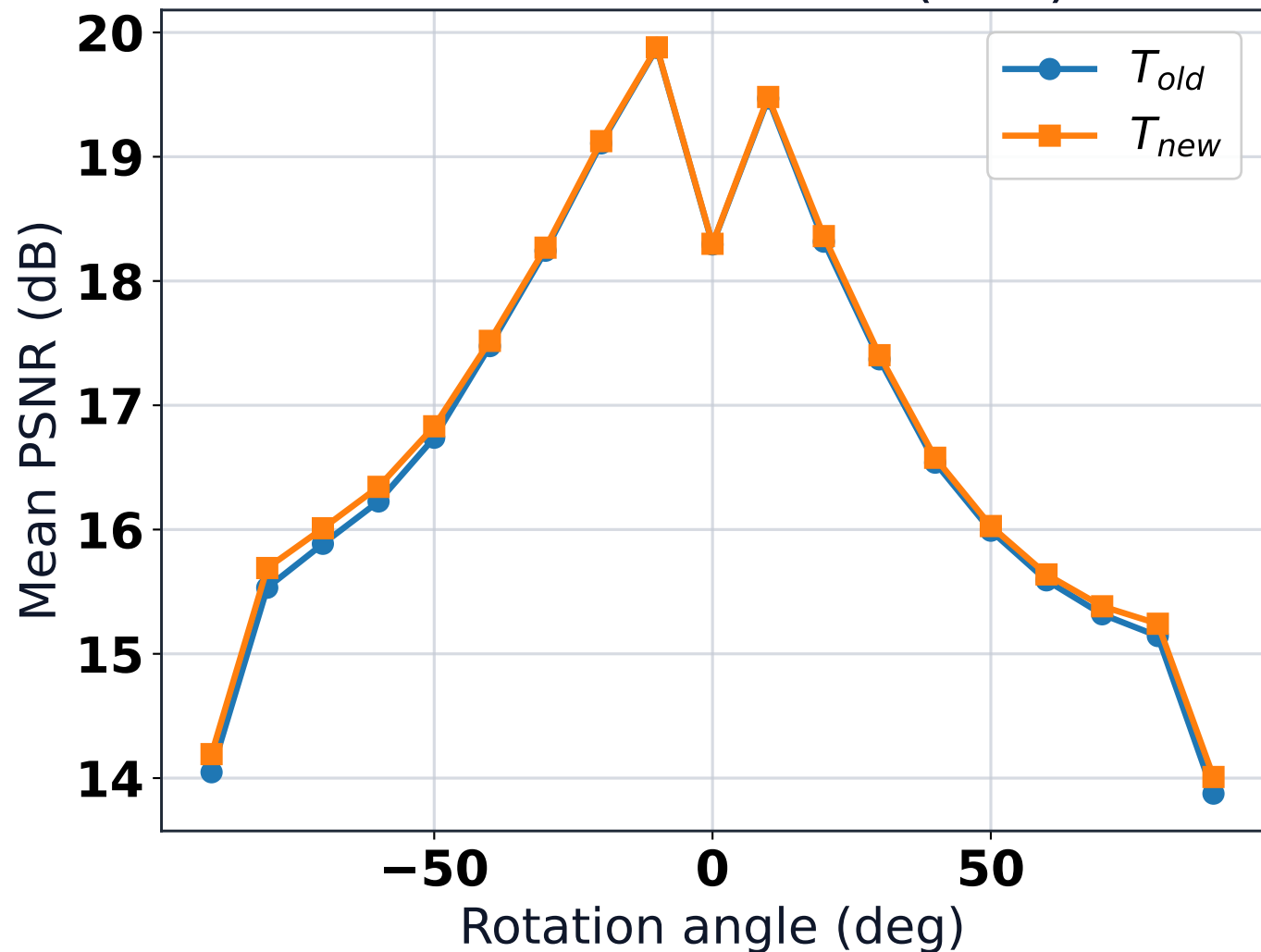
Robustness: PSNR (test)
