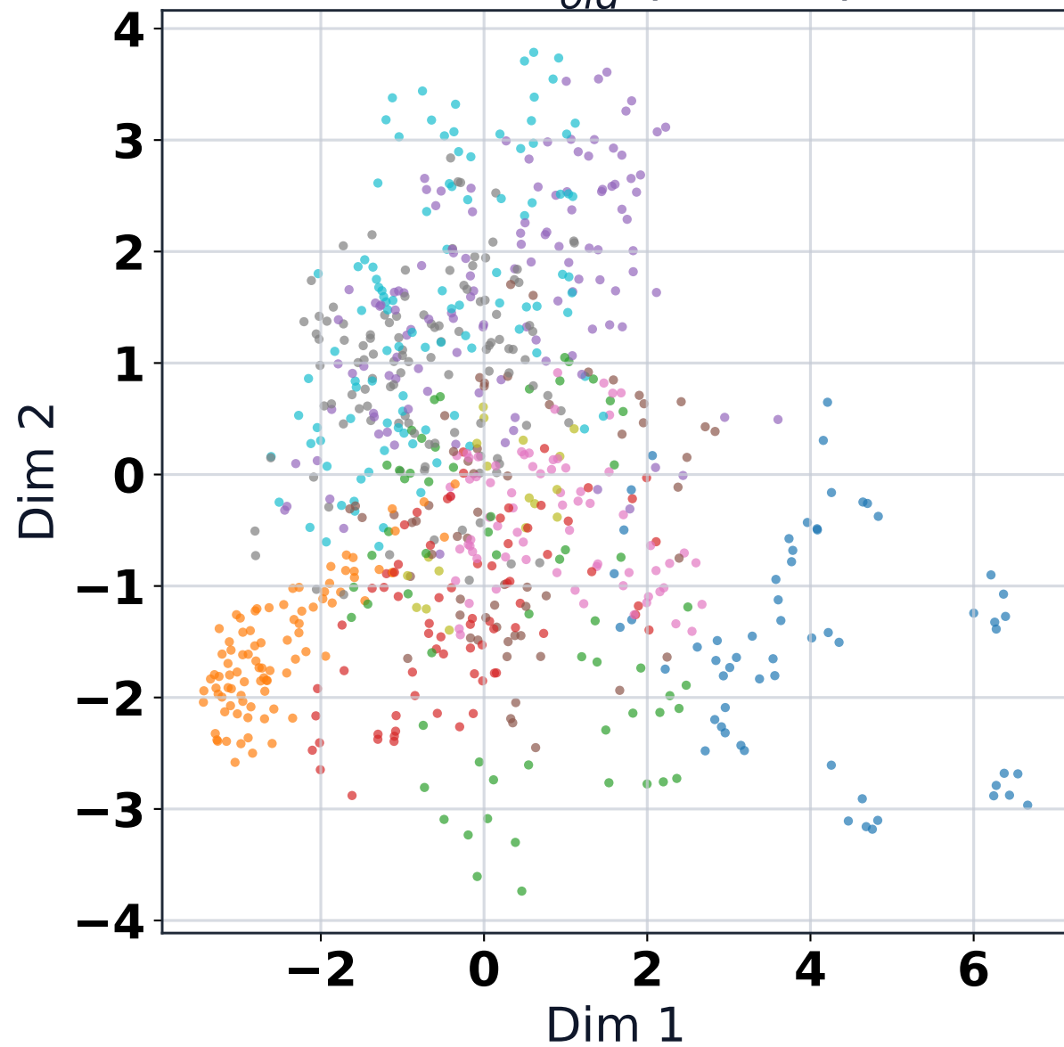
PCA: B_{old}^* (Chaos)
