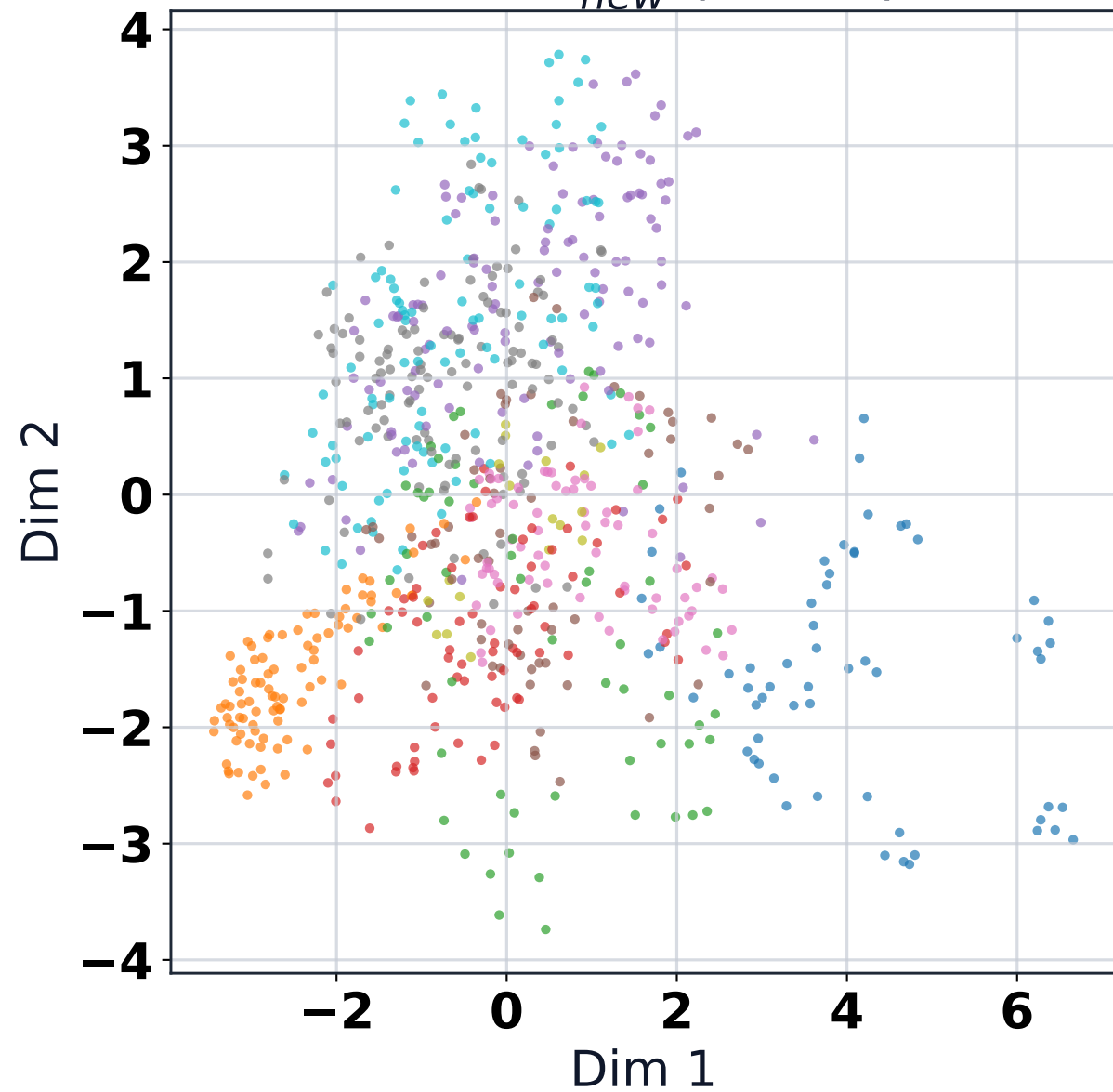
PCA: B_{new}^* (Order)
