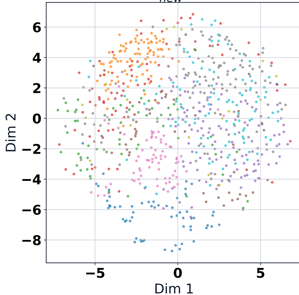
MDS: B_{new}^* (Order)
