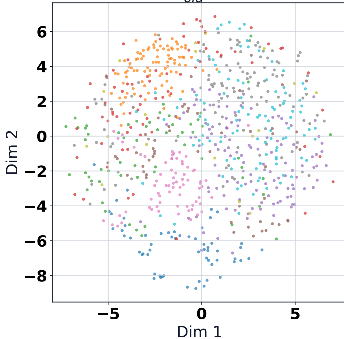
MDS: B_{old}^* (Chaos)
