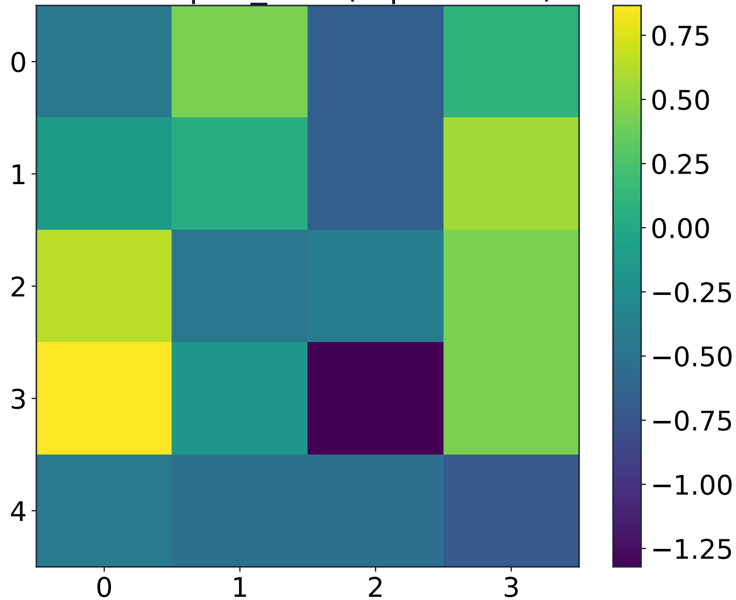
Heatmap: T_{\text{new}} (Equivariant)
