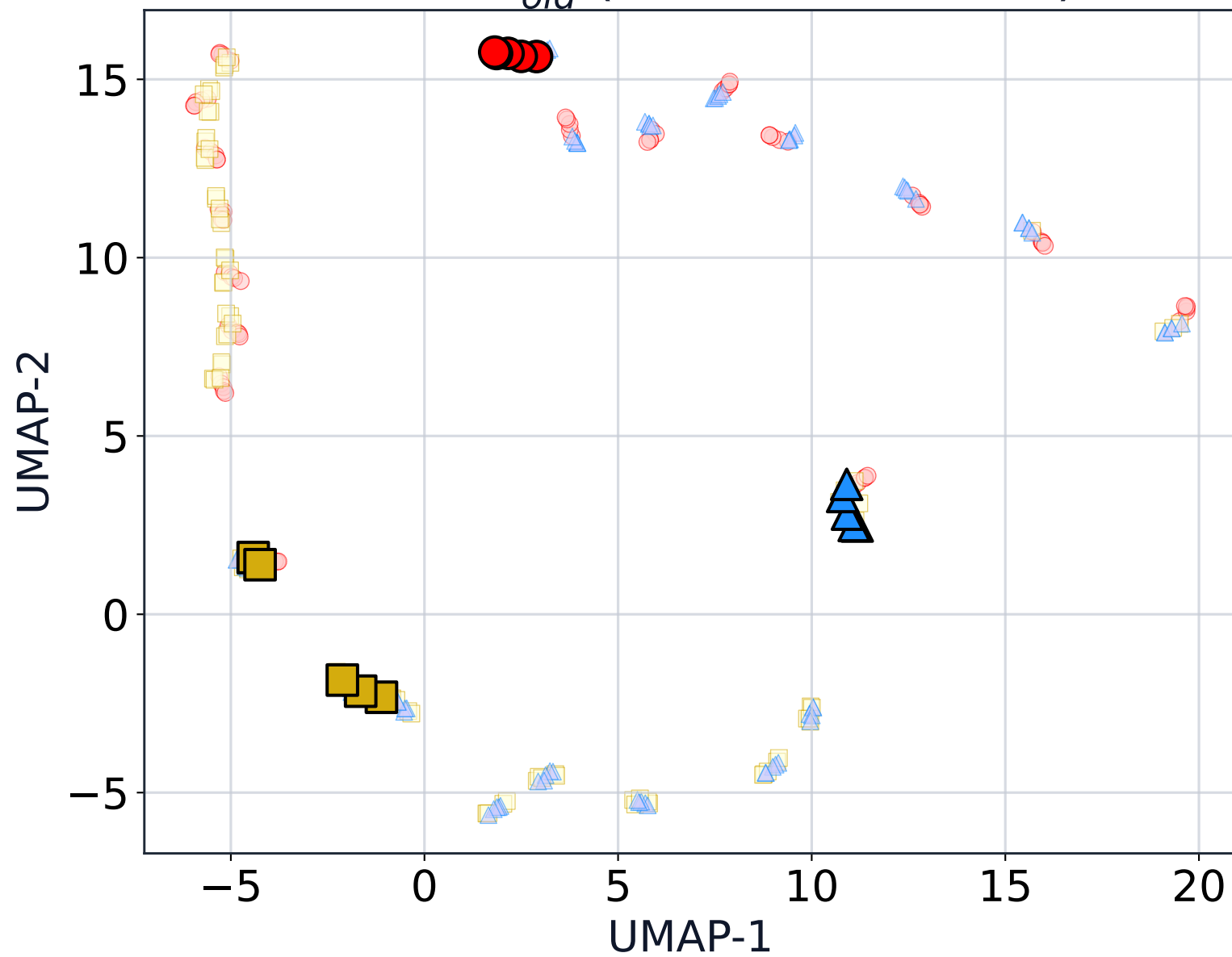
UMAP: B_{old}^* (Rotated vs Static)
