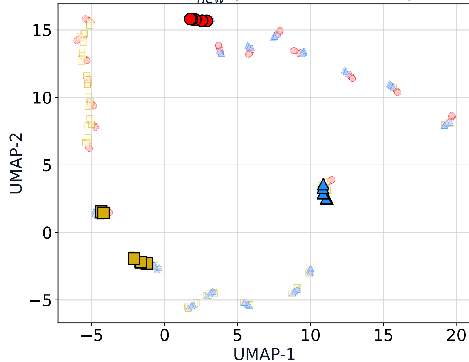
UMAP: B_{new}^* (Rotated vs Static)
