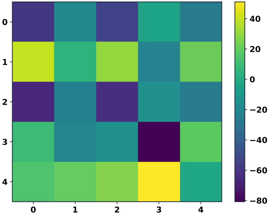
Heatmap: J^A
