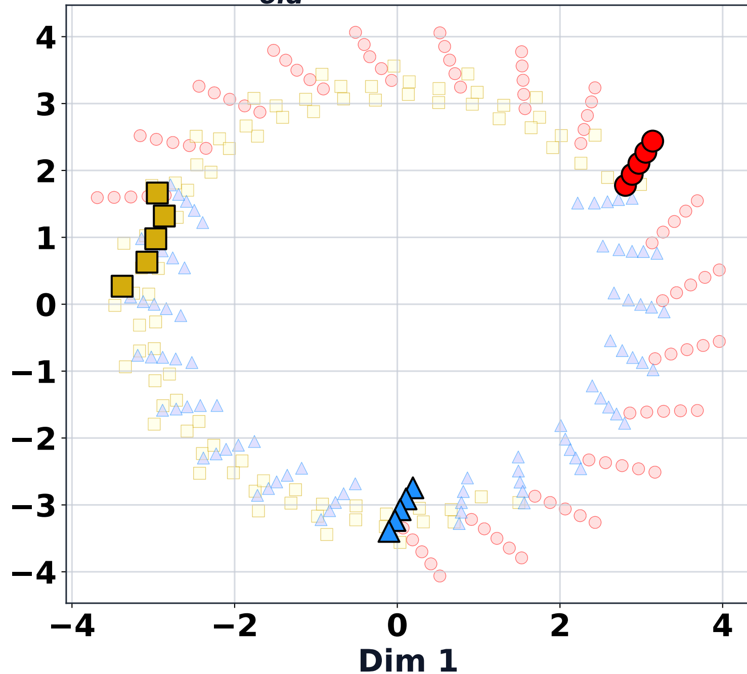
MDS: B_{old}^* (Rotated vs Static)
