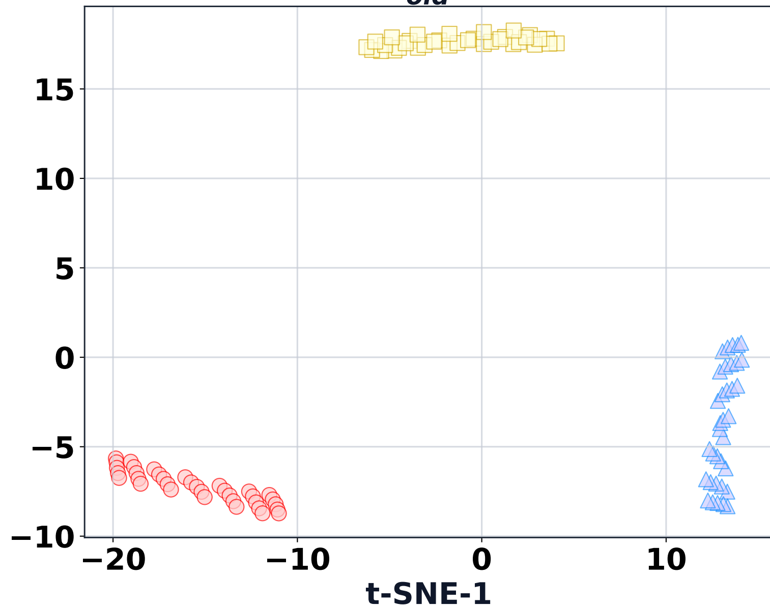
t-SNE: B_{old}^* (Chaos)
