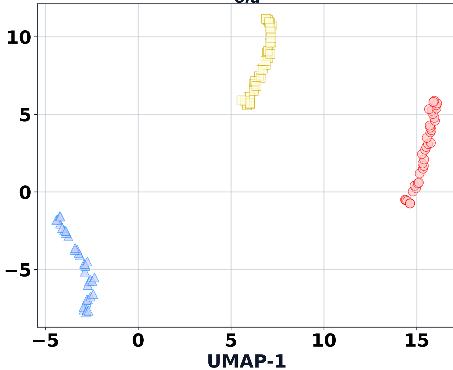
UMAP: B_{old}^* (Chaos)
