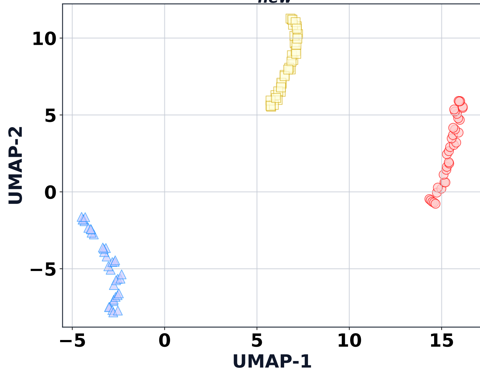
UMAP: B_{new}^* (Order)
