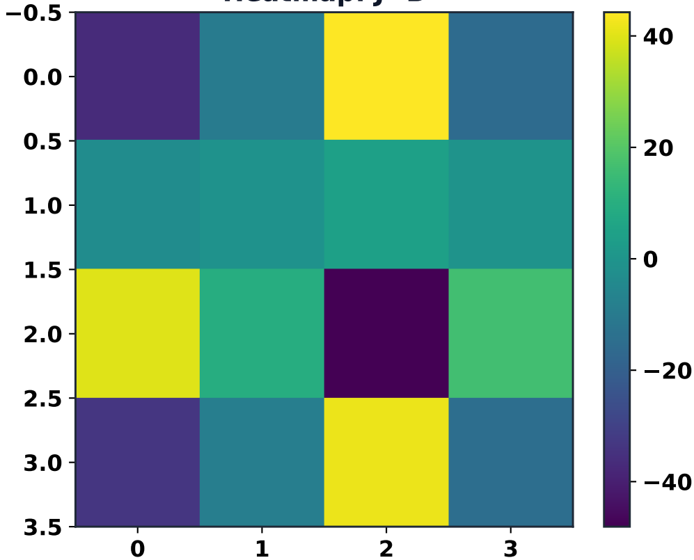
Heatmap: J^B
